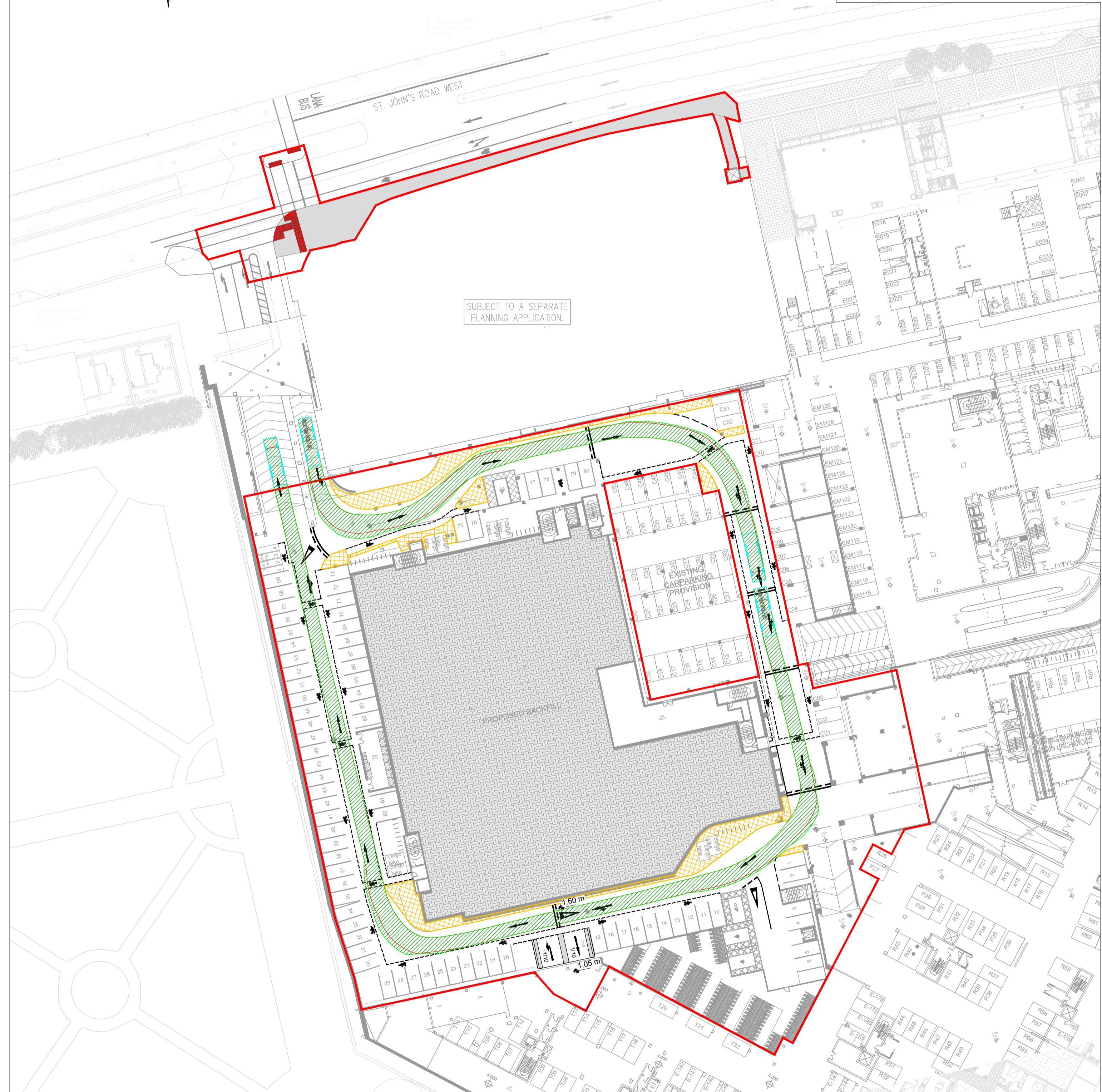
SWEPT PATH ANALYSIS-REFUSE VEHICLE, BASEMENT LEVEL. SCALE 1:500
